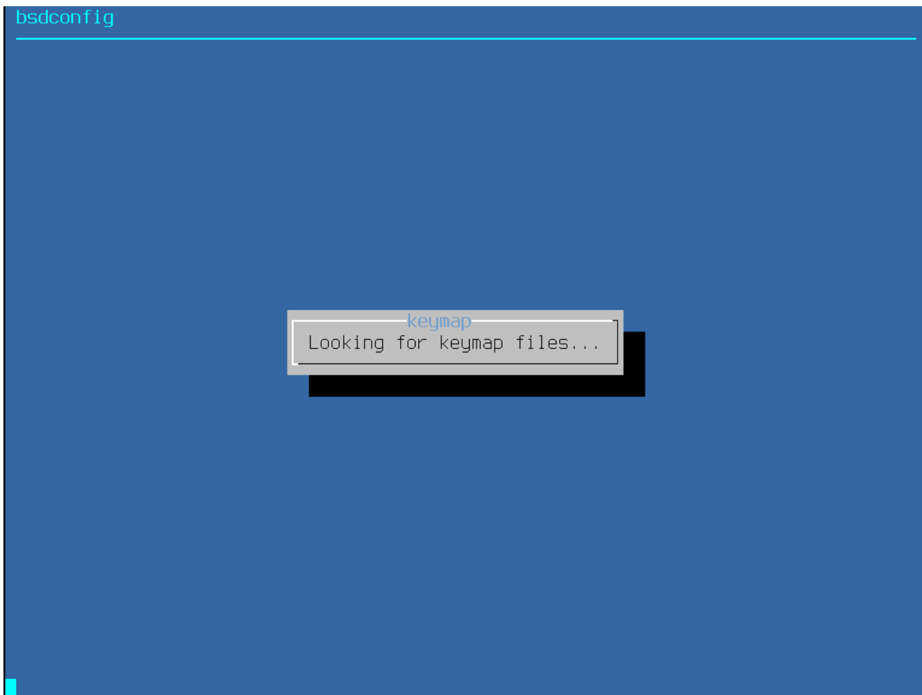
Figure 4. Keymap Loading
