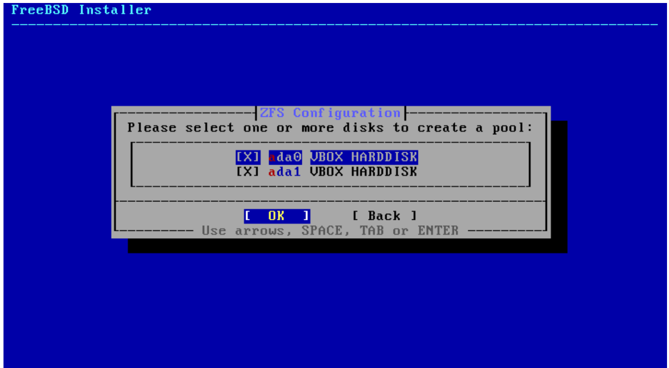
Figure 22. Disk Selection
